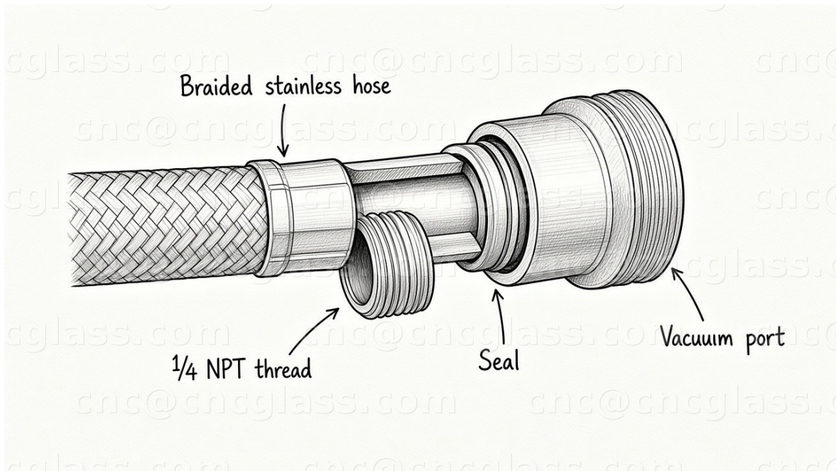
1/4 NPT connection (hand-drawn sketch): braided stainless hose with 1/4 NPT thread into vacuum port — seal detail.
