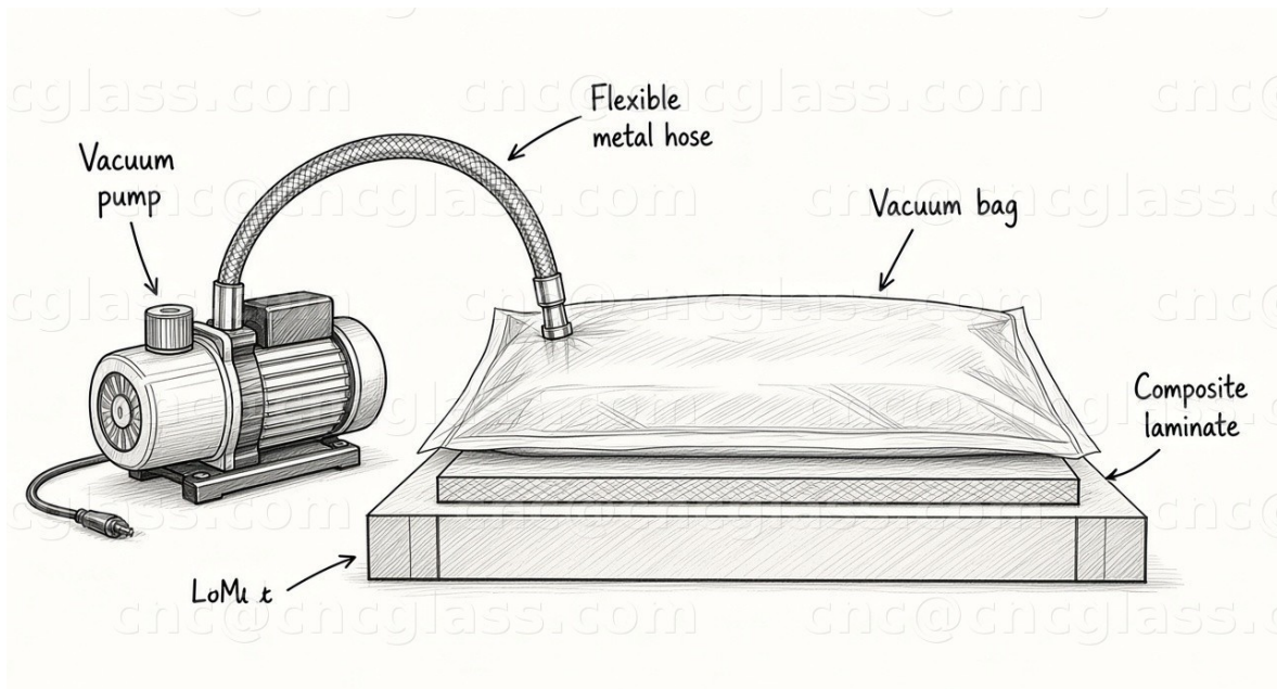
Vacuum process line (hand-drawn sketch): CNCGLASS flexible metal hose links vacuum pump to bagged composite laminate.
