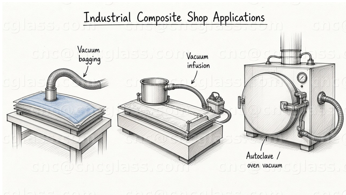
Shop applications (hand-drawn sketch): vacuum bagging, vacuum infusion, and autoclave / oven vacuum lines.
