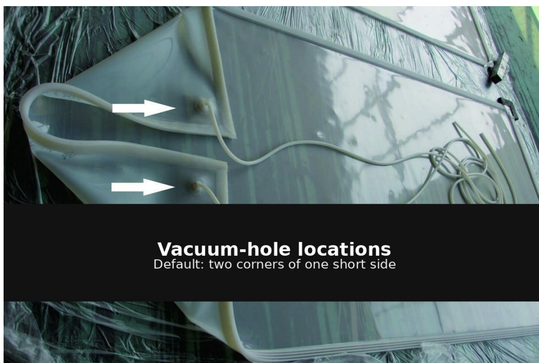
Vacuum-hole locations — default: two corners of one short side (customizable)
