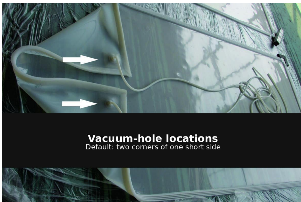
Vacuum-hole locations — default: two corners of one short side
