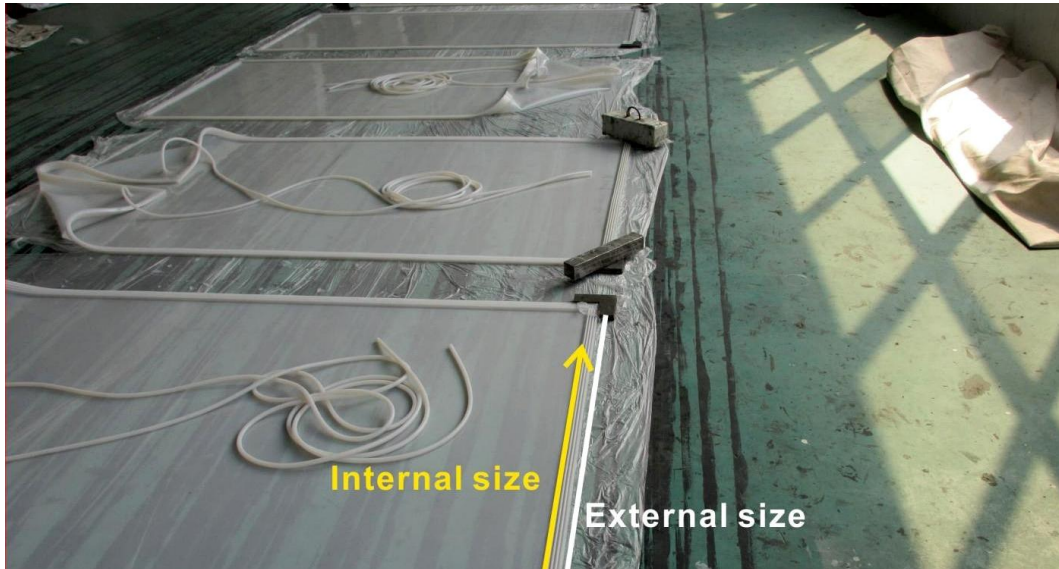
Silicone vacuum bags (two sheets with edge sealing) — Internal size / External size
