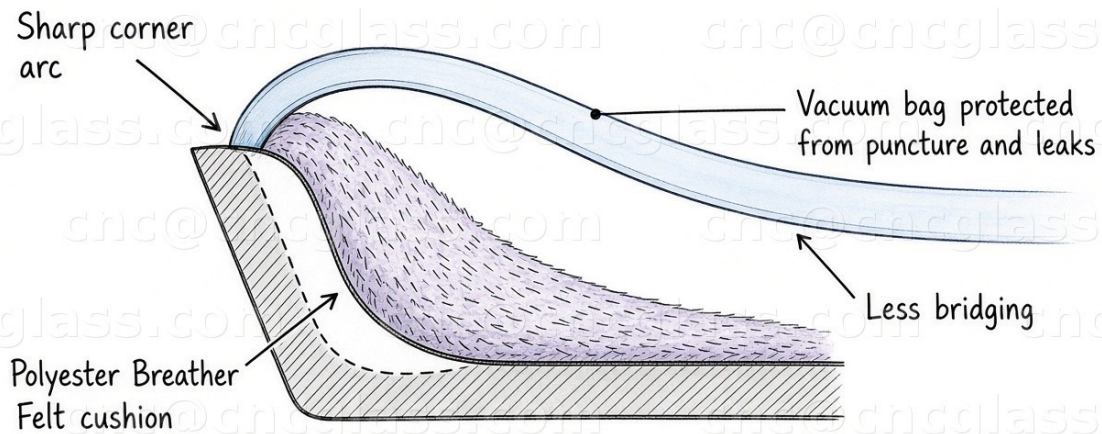
Corner cushioning (hand-drawn sketch): polyester breather felt pads sharp corners and arcs — protects the vacuum bag from puncture and leaks; less bridging.
