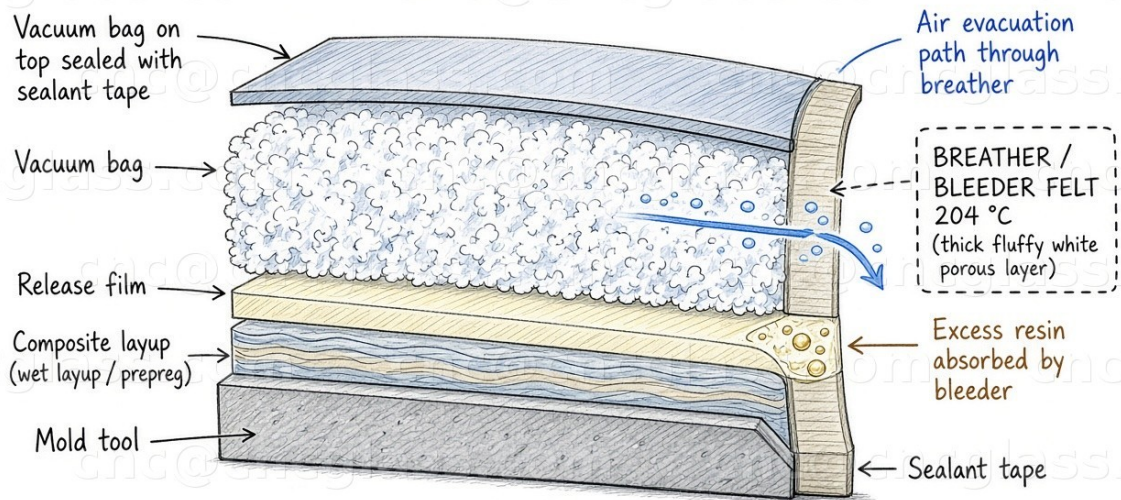
Vacuum bag stack (hand-drawn sketch): polyester breather / bleeder felt position under the vacuum bag — service up to 204 °C; air path and excess-resin absorption.
