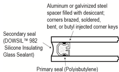
Figure 1: Dual-Seal Type
